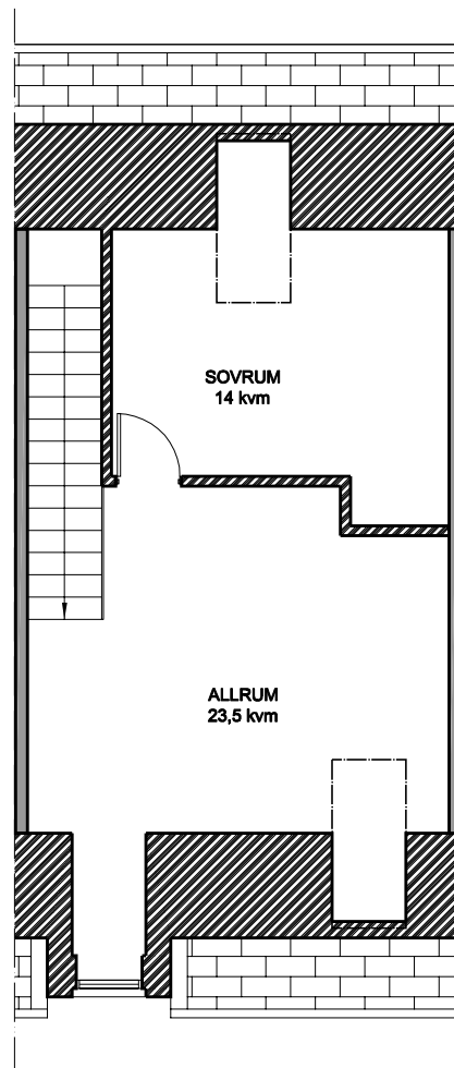
PLAN 3
